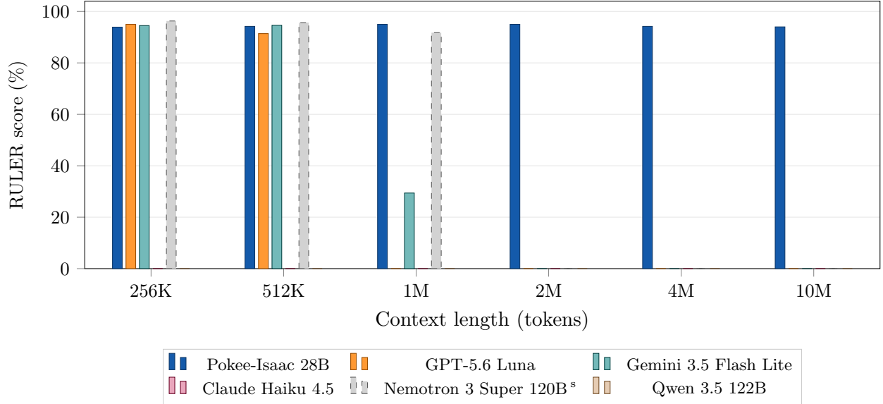
Figure 1: RULER score by context length. Pokee-Isaac 28B is the only one that sustains beyond 1M context. Nemotron 3 Super 120B’s bars at 256K–1M (dashed outline) are NVIDIA’s self-reported figures; from 2M onward that series is our own and is zero.
